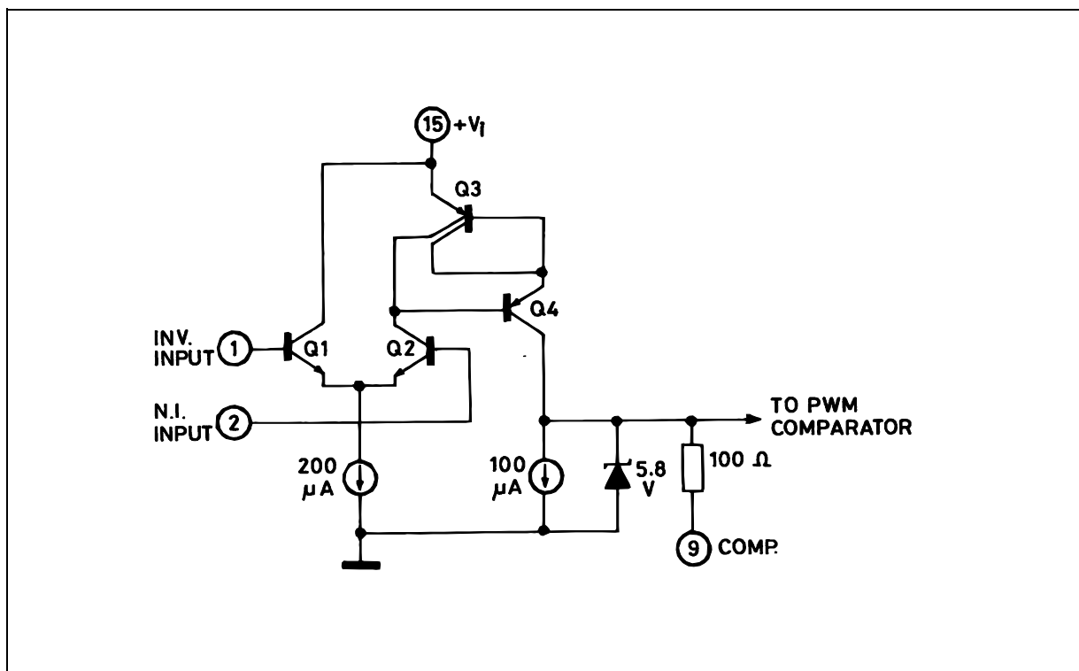
Figure 5 : Error Amplifier.
