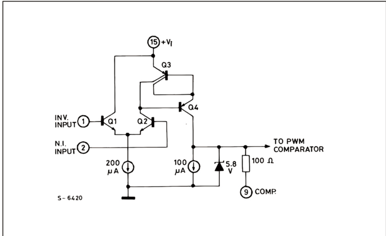
Figure 5 : Error Amplifier.
