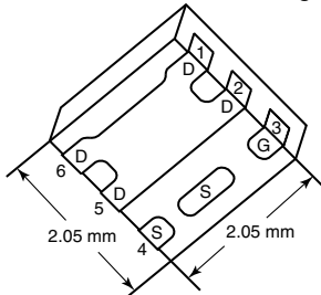
PowerPAK SC-70-6L-Single
