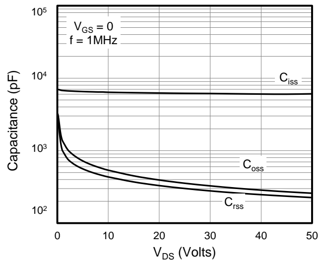
Figure 4: Capacitance Characteristics
