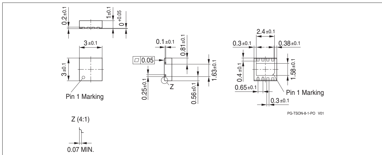
Figure 20 PG-TSON-8 (Plastic thin small outline nonlead PG-TSON-8) 1)
