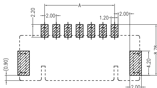
PCB LAYOUT(Tolerance:±0.05)
