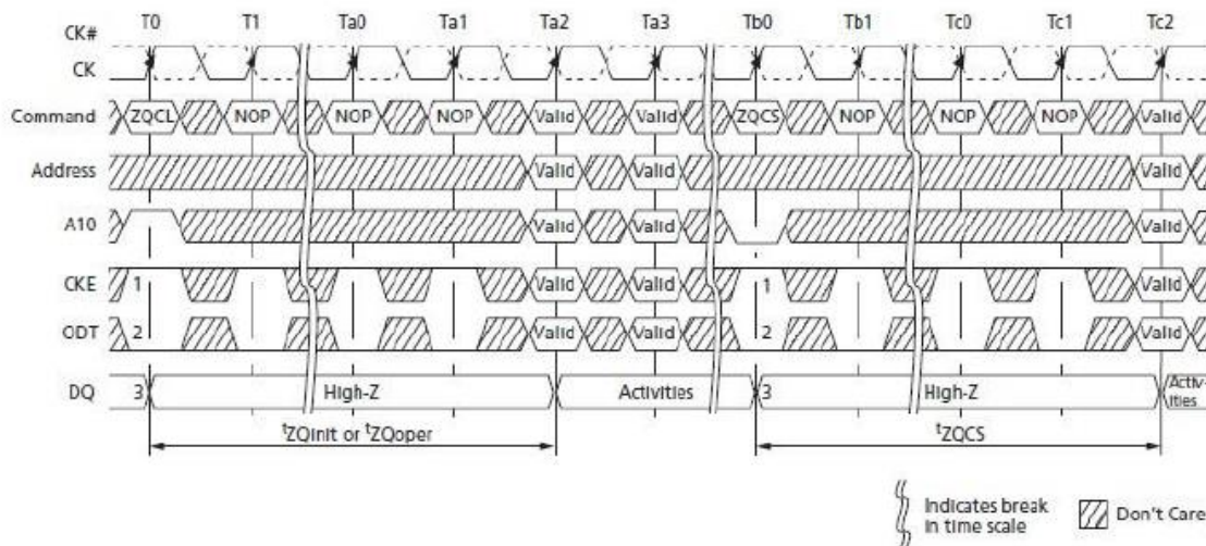
ZQ CALIBRATION Timing (ZQCL and ZQCS)
