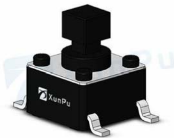
TS-1002ST W6.00xD6.00xH7.30
