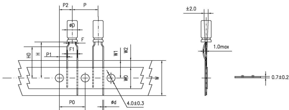
DIMENSIONS(mm)
