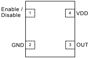
Figure 1. Pin Assignments
