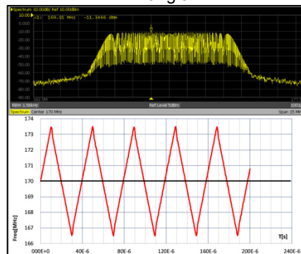
Triangle
