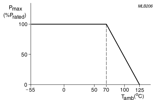
Fig. 6 Maximum dissipation ( P_{\max} ) in percentage of rated power as a function of the operating ambient temperature ( T_{\text{amb}} )
