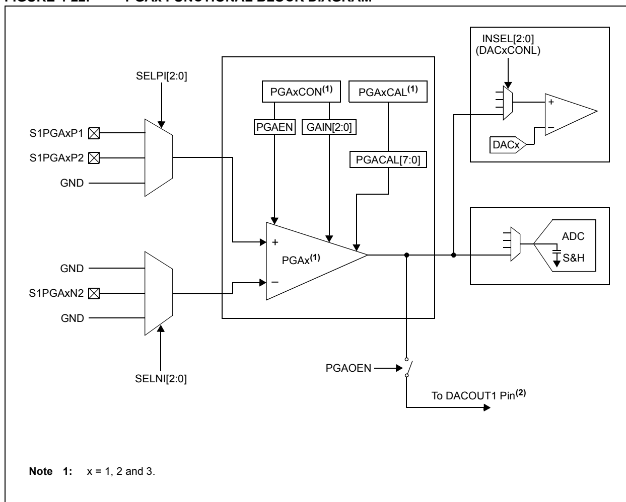
FIGURE 4-22: PGAx FUNCTIONAL BLOCK DIAGRAM
