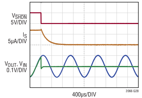
Shutdown Transient with Sinusoidal Input
