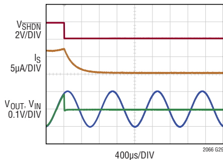
Shutdown Transient with Sinusoidal Input
