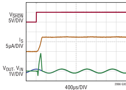
Enable Transient with Sinusoidal Input
