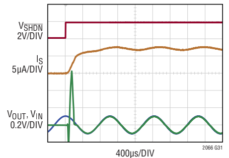
Enable Transient with Sinusoidal Input
