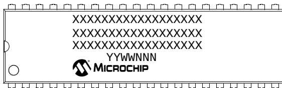
40-Pin PDIP
