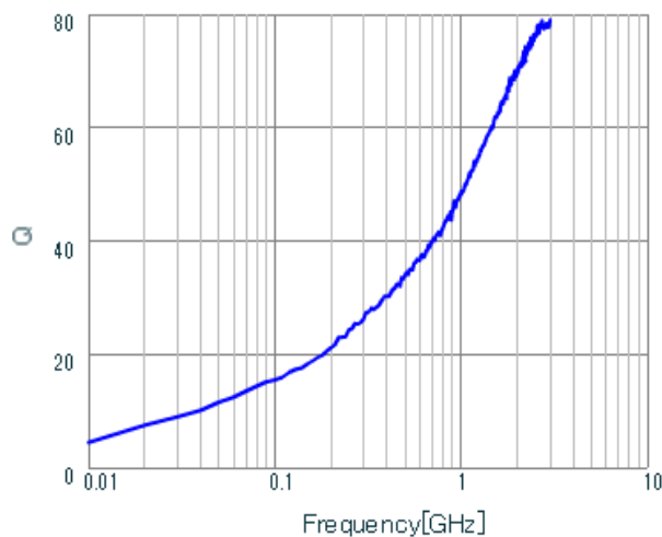
Q-Frequency Characteristics
