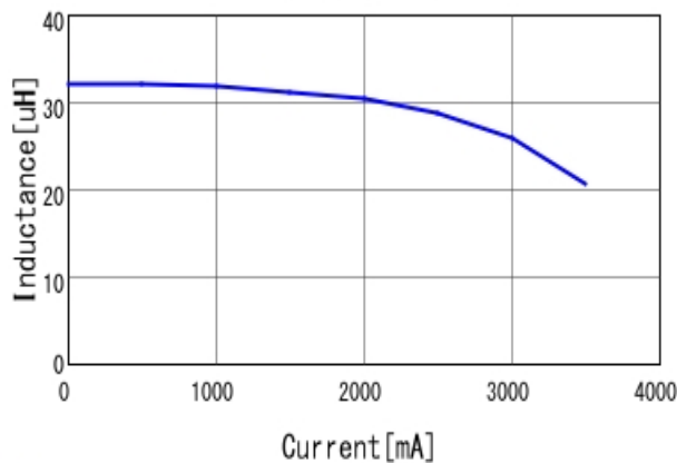
■ DEM8045Z-330M L-Current 20degC
