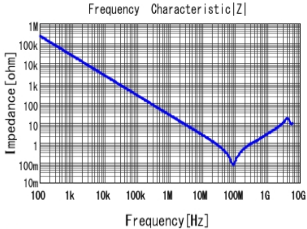
■ GRM216R71H682KA01 |Z| DC0V, 25degC
