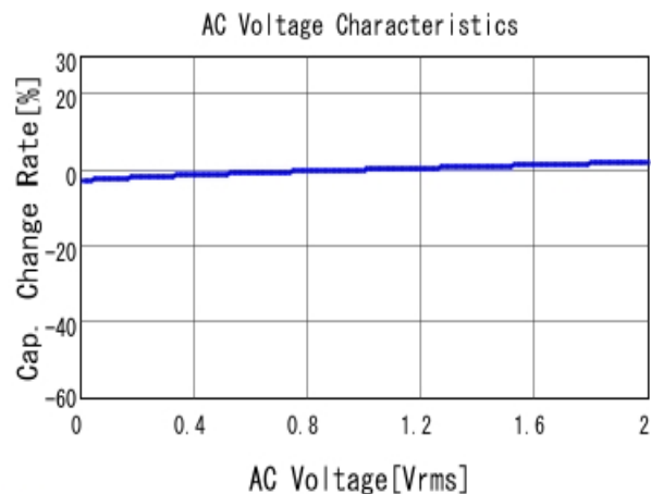
■ GRM216R71H682KA01 C-AC Voltage capchange, DC0V, 25.0d
