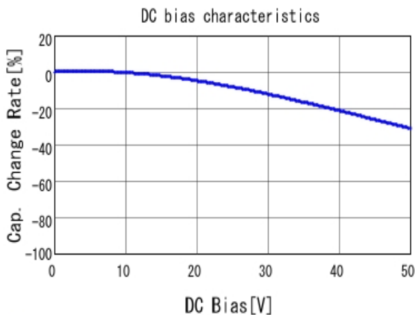
■ GRM216R71H682KA01 C-DC bias capchange, 25.0degC, AC1.
