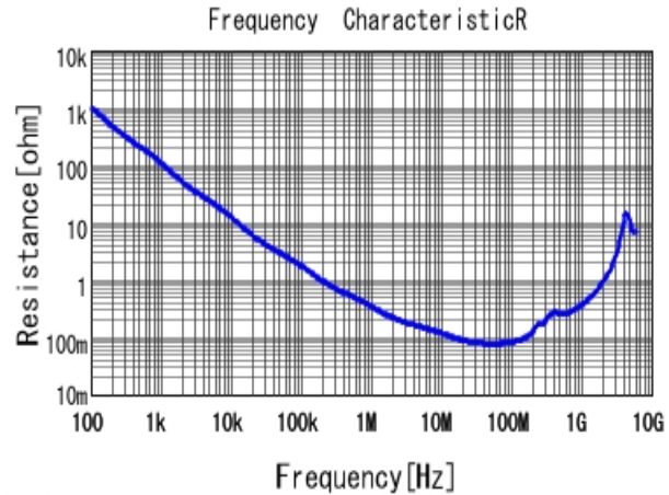
■ GRM216R71H682KA01 R DC0V, 25degC
