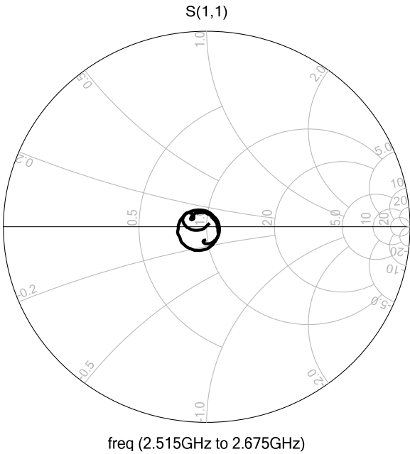
Figure7. S11
