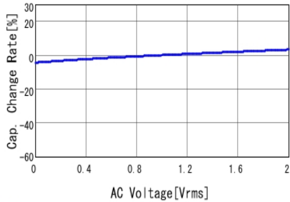
■ RDER71H105K2K1H03B C-AC Voltage capchange, DC0V, 25.0
