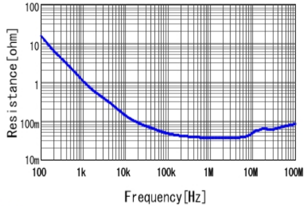
■ RDER71H105K2K1H03B R DC0V, 25degC
