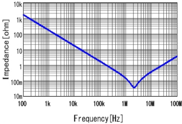
■ RDER71H105K2K1H03B |Z| DC0V, 25degC
