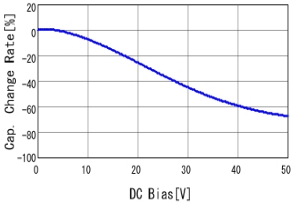
■ RDER71H105K2K1H03B C-DC bias capchange, 25.0degC, AC1
