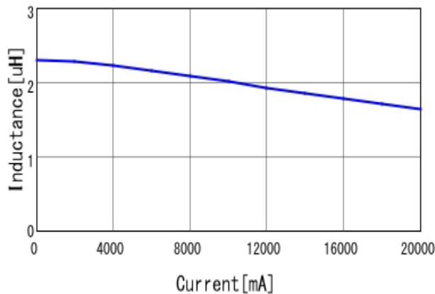
DFEG10040D-2R2M L-Current 20degC
