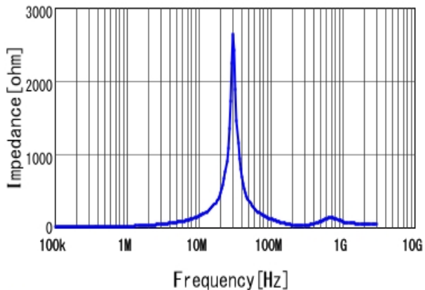
DFEG10040D-2R2M |Z|
