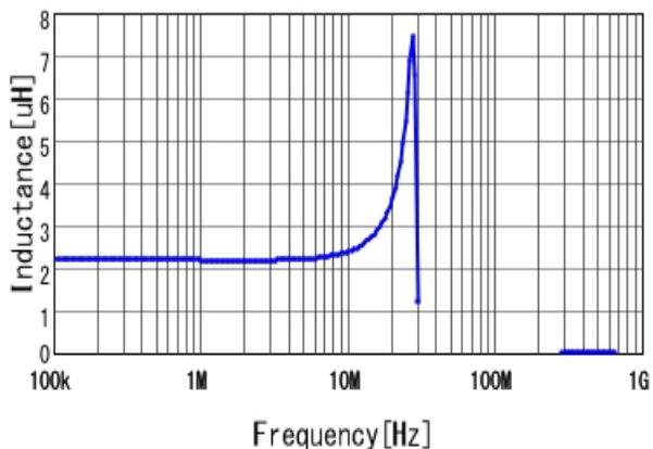
DFEG10040D-2R2M L
