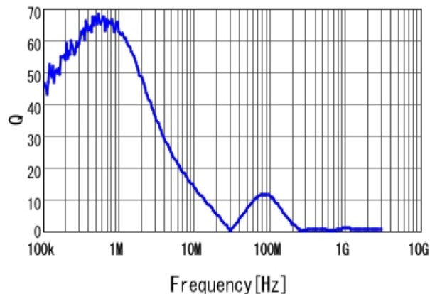
DFEG10040D-2R2M Q
