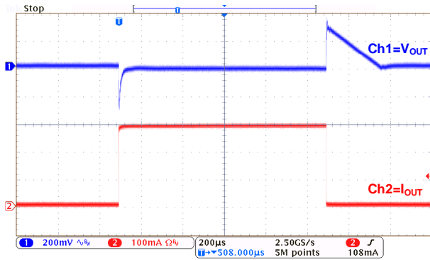
Load Transient: MD8333 ( I_{OUT}=1mA\sim 300mA\sim 1mA )
