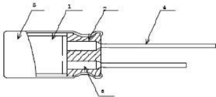
Fig. 1 Cross-section view
