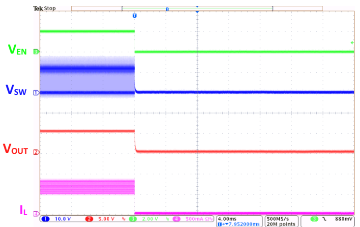
Figure 18. Shutdown Through EN, I_{OUT}=0.6A
