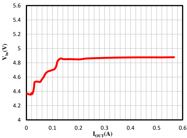
Figure 5. V_{BS} vs. I_{OUT}
