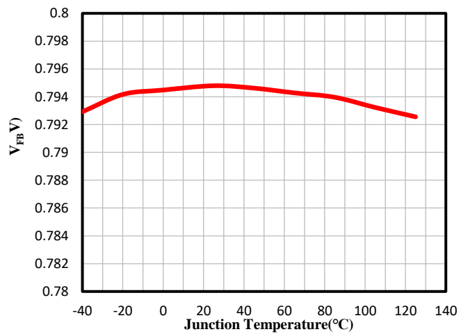
Figure 6. V_{FB} vs. Junction Temperature
