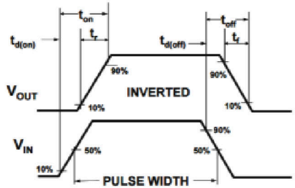
Figure8. Switching wave
