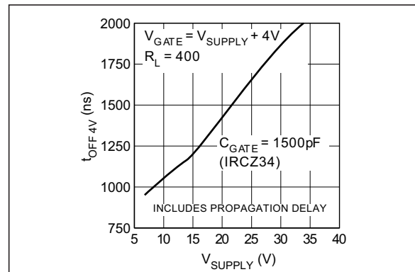
FIGURE 3-6: Gate Turn-Off Delay vs. Supply Voltage.
