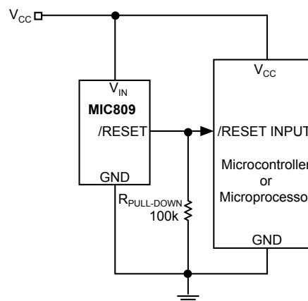
Figure 2. Ensuring a Valid \overline{\text{RESET}} Signal at Low Voltage
