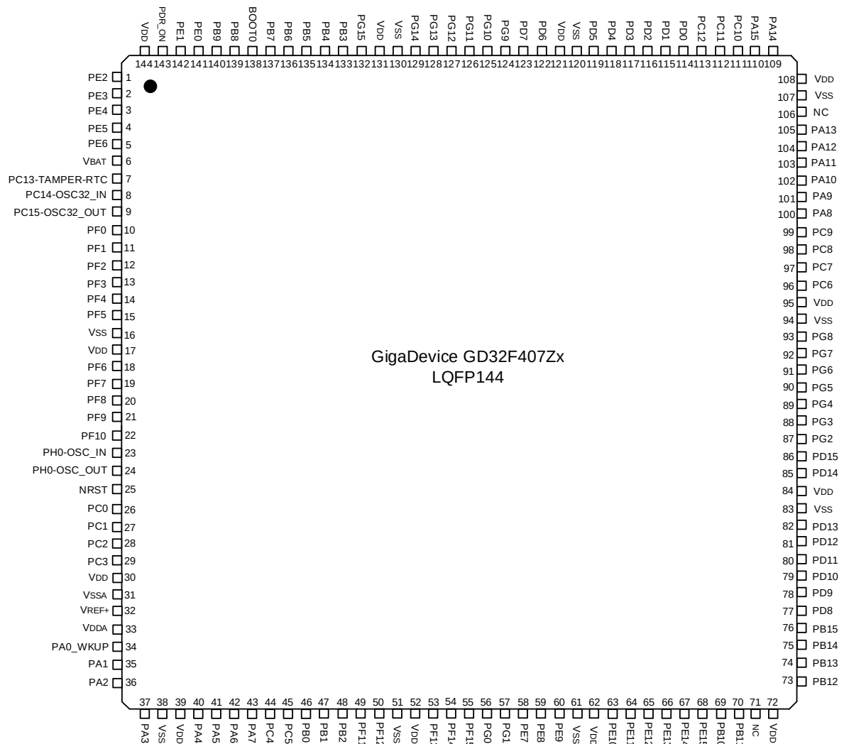
Figure 4. GD32F407Zx LQFP144 pinouts
