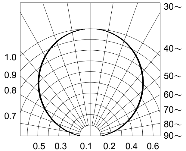
Fig.6-Radiation Diagram Ta=25-C 0~ 10~ 20~
