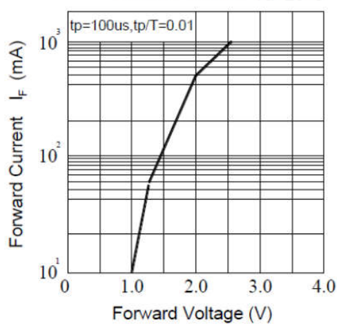
Fig.3-Forward Current vs. Forward Voltage T_a=25^{\circ}\text{C}
