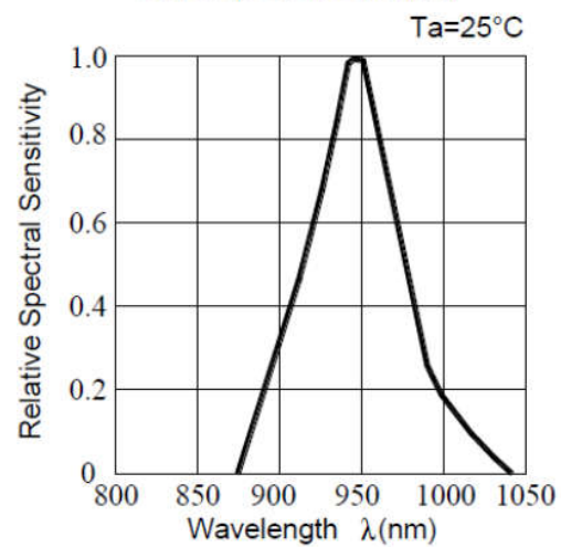
Fig.2-Spectral Sensitivity
