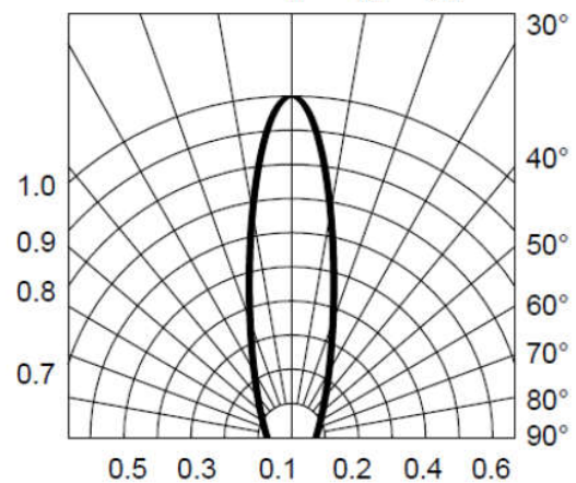
Fig.4-Radiation Diagram T_a=25^{\circ}\text{C}
