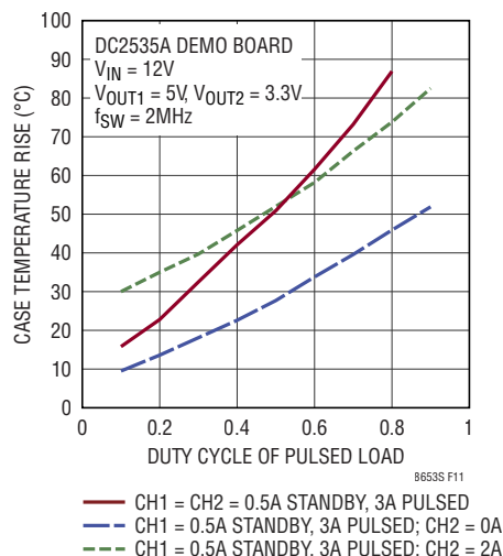
Figure 11. Case Temperature Rise vs. 3A Pulsed Load
