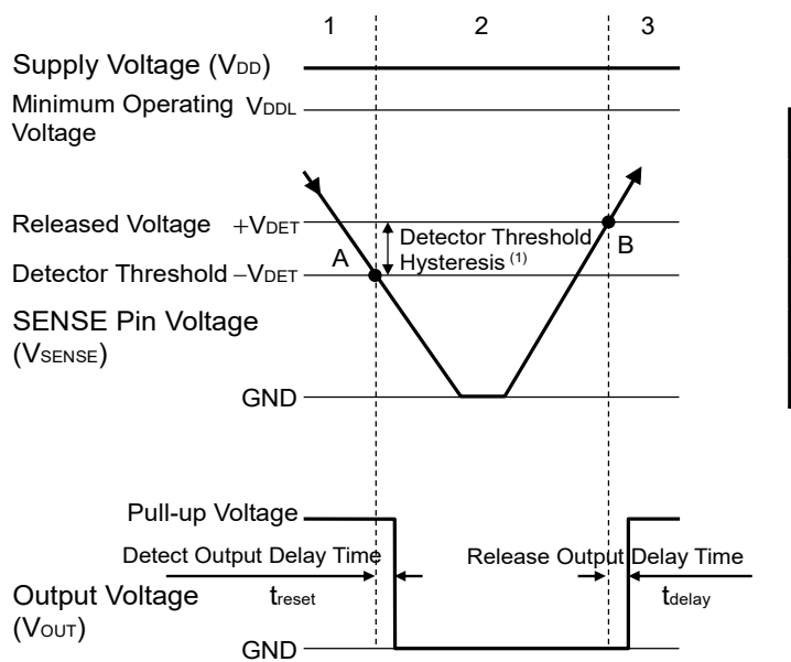
Operation Diagram
