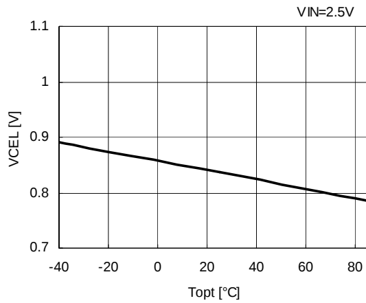
3) CE "L" Input Voltage vs. Temperature R1283x00xx
