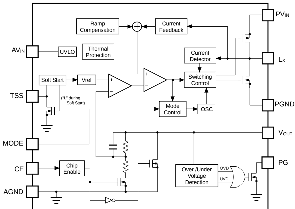
RP506Kxx1B/E Block Diagram
