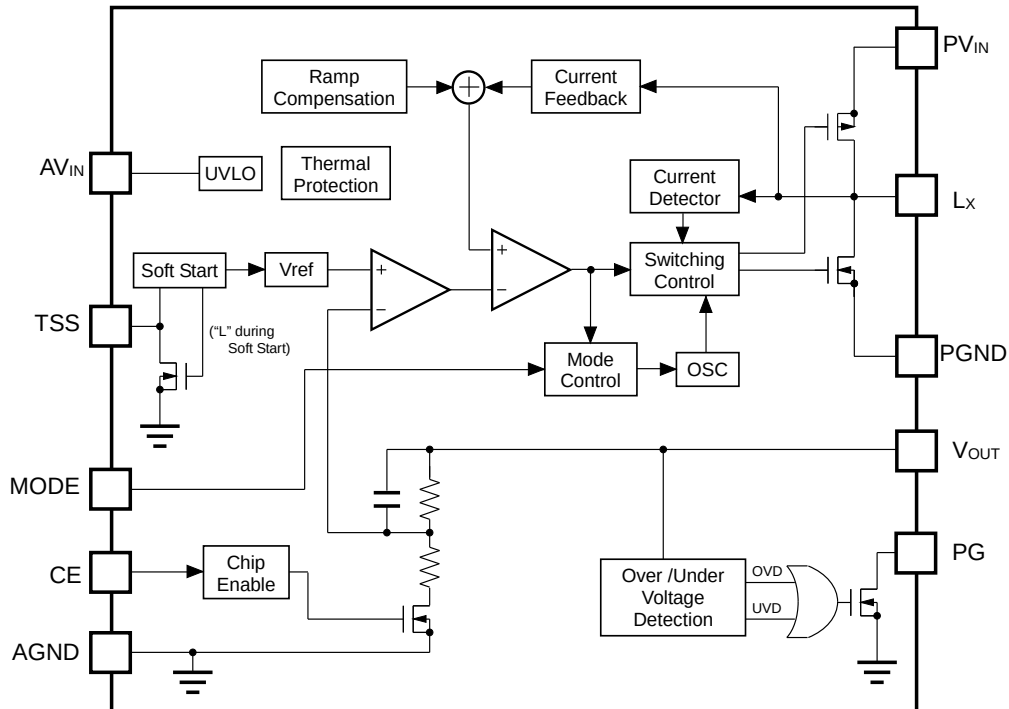
RP506Kxx1A/D Block Diagram
