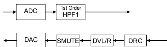
Figure 32. Path at Recording Mode 2 &amp; Playback Mode 2
