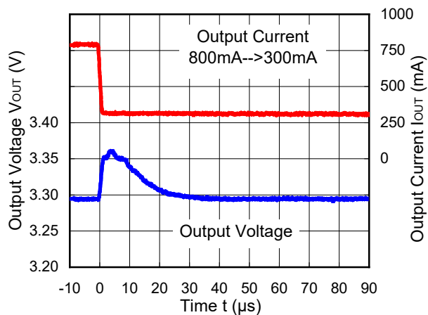
RP505K331A/B ( V_{IN}=5.0V )
