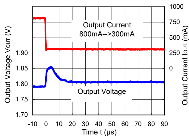
RP505K181A/B ( V_{IN}=3.6V )
