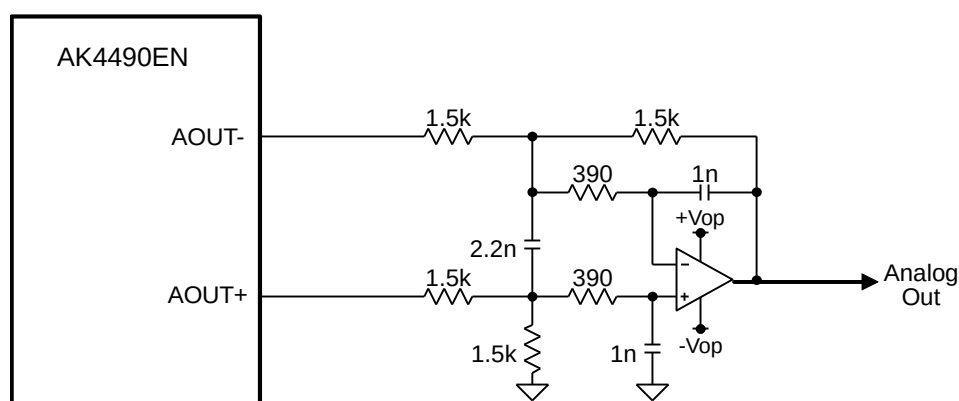
Figure 40. External LPF Circuit Example 1 for PCM ( f_c = 99.2kHz , Q=0.704 )
