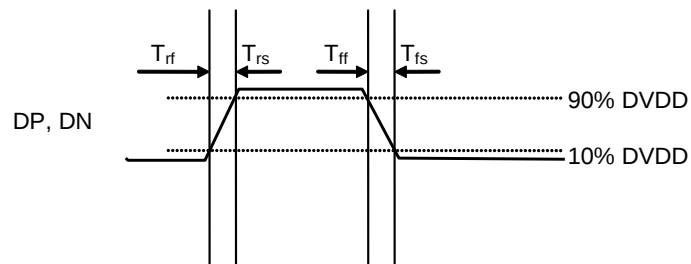
Figure 4. Rise/Fall Time
