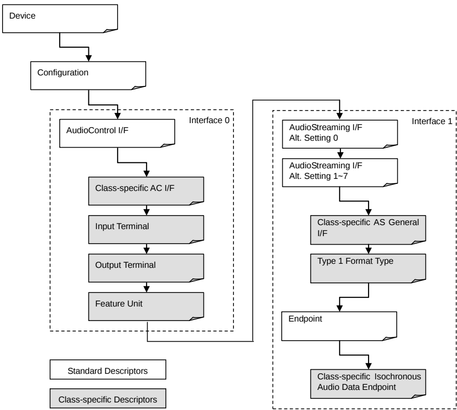
Figure 17. Descriptor Hierarchy
