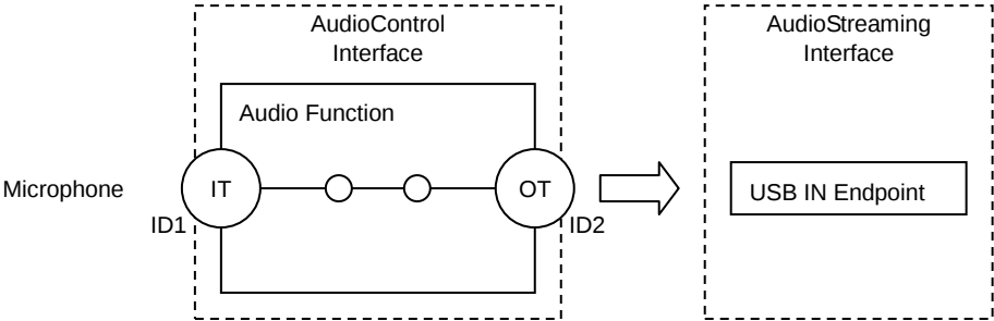
Figure 16. AK5374 Topology
