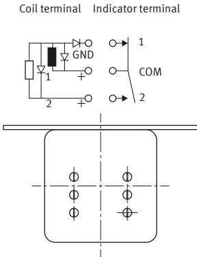
Solder terminal layout Latching
