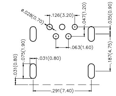
Recommended P.C.Board Layout General Tolerances: ±0.05mm
