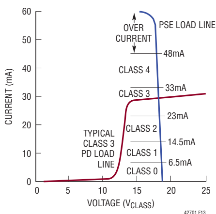
Figure 13. PD Classification
