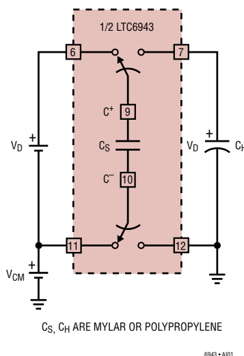
Figure 1. Differential to Single-Ended Converter
