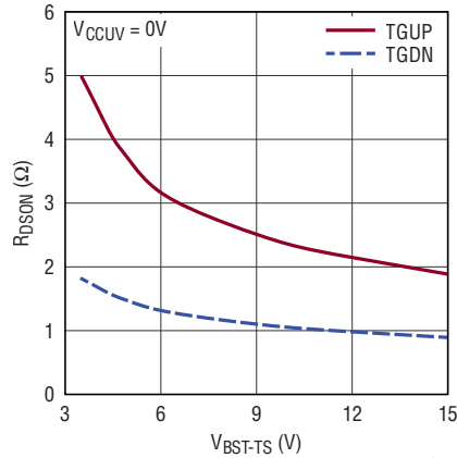
Driver On Resistance vs V_{BST-TS} Voltage
