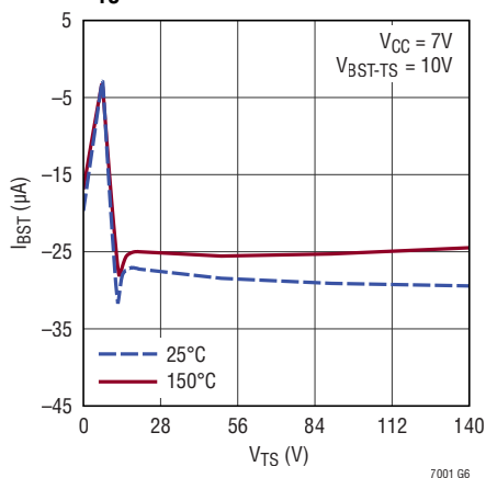
Charge Pump Output Current vs V_{TS}
