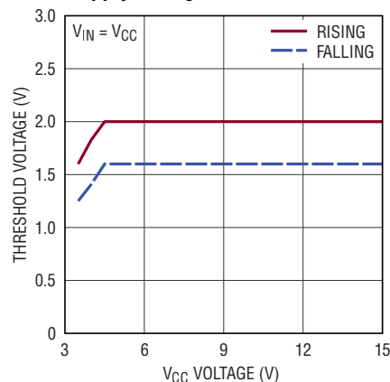
Input Threshold Voltage vs V CC Supply Voltage
