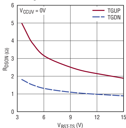
Driver On Resistance vs V BS -TS Voltage
