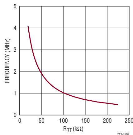
Figure 2. R RT vs Frequency
