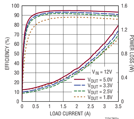
Efficiency & Power Loss vs Load Current at 1MHz
