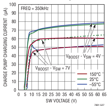
BOOST Charge Pump Charging Current vs SW Voltage
