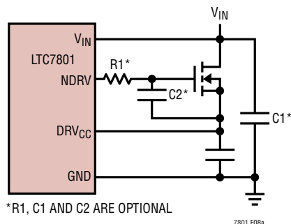
(8a). Configuring the NDRV LDO
