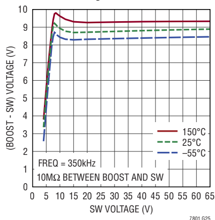
Boost Charge Pump Voltage vs SW Voltage
