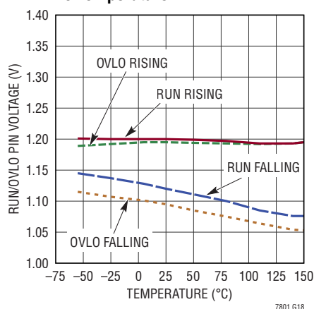
RUN/OVLO Threshold vs Temperature
