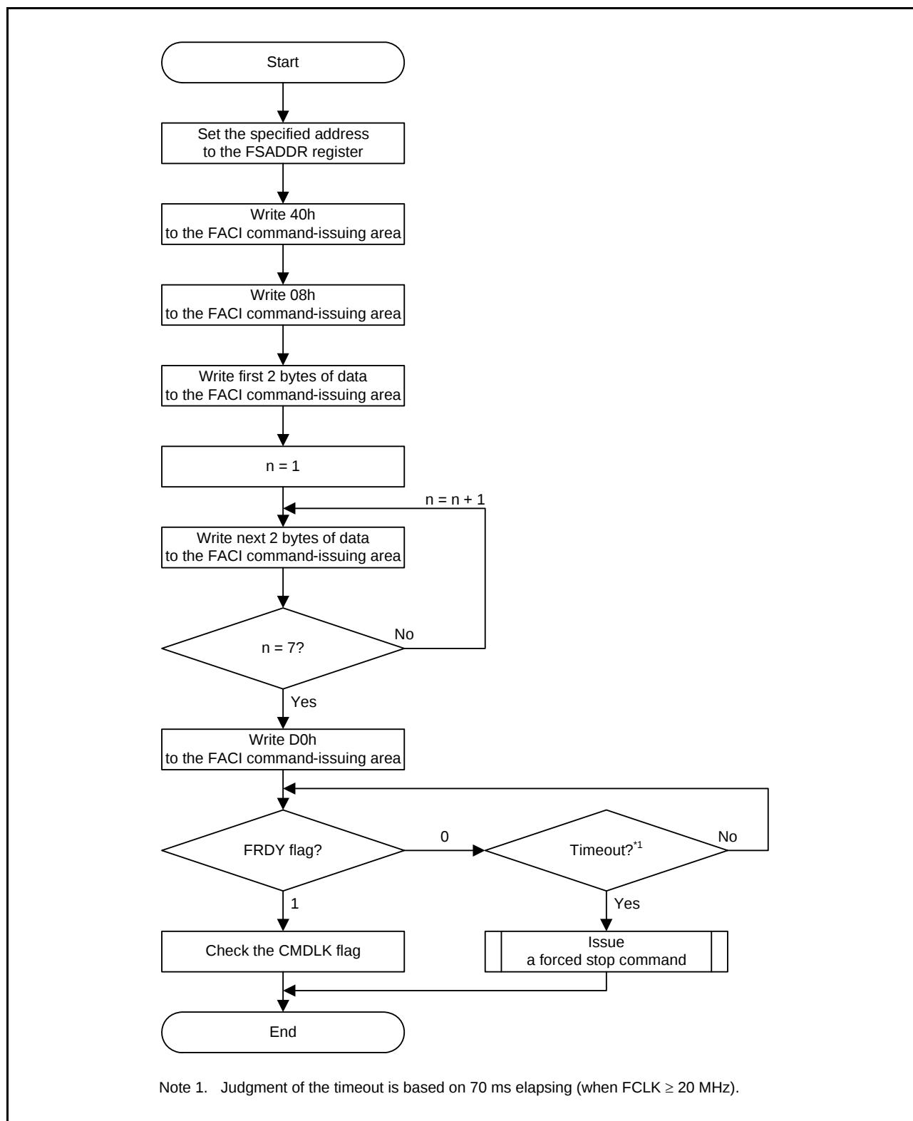
Figure 6.19 Usage of the Configuration Set Command
