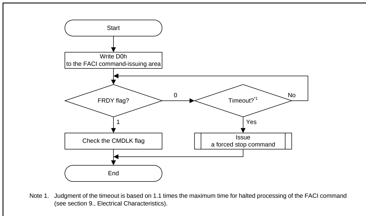
Figure 6.15 Usage of the P/E Resume Command
