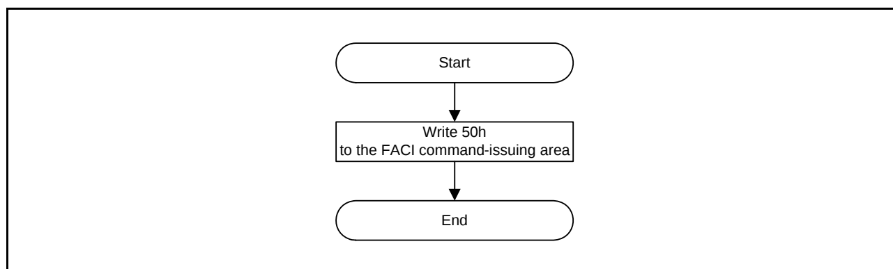
Figure 6.16 Usage of the Status Clear Command
