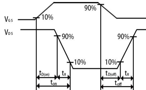
Figure 17. Switching Time Waveform
