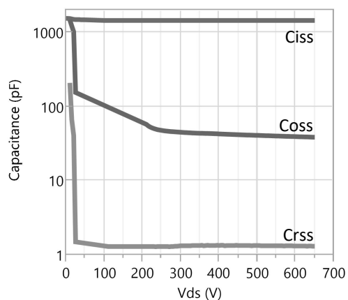
Figure 5. Typical Capacitance
